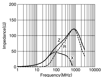
MPZ1608Y221B
