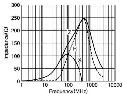
MPZ1608Y151B
