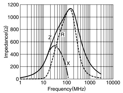
MPZ1608S102A
