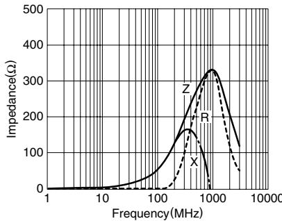
MPZ1608D600B
