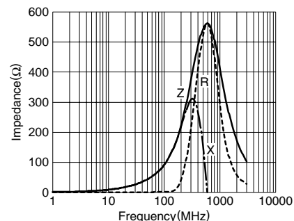
MPZ1608D101B
