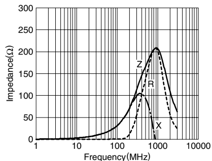
MPZ1608D300B
