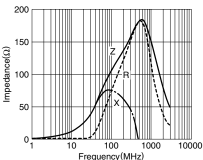
MPZ1608Y101B
