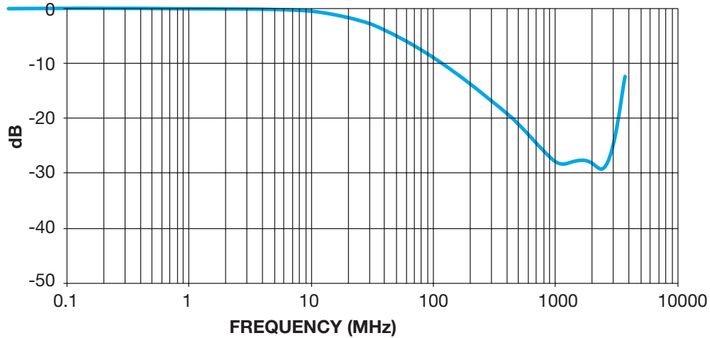
Preliminary AVX W3F45C2218AT Typical Far-side XTALK Elements 1 - 2
