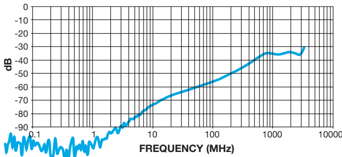
Preliminary AVX W3F45C4718AT Typical Far-side XTALK Elements 1 - 4
