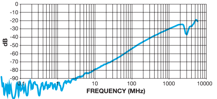
Preliminary AVX W2F43A4708AT Typical Far-side XTALK Elements 1 - 3
