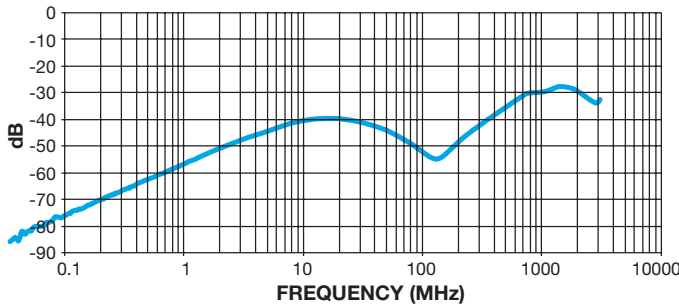
Preliminary AVX W3F45C4718AT Typical Far-side XTALK Elements 1 - 2
