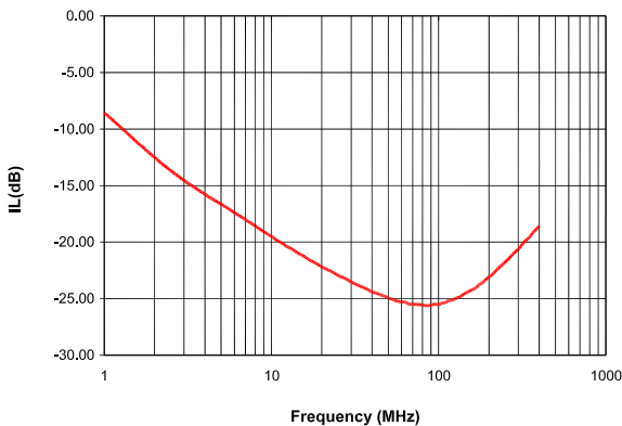
Typical Insertion Loss @ 50 ohm
