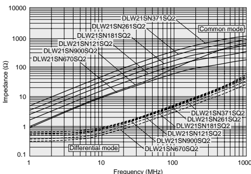
DLW21SN_SQ2 Series
