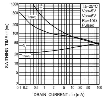
Fig.20 Switching characteristics
