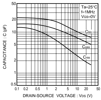
Fig.18 Typical capacitance vs. drain-source voltage
