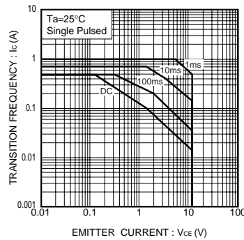
Fig.8 Safe operation area
