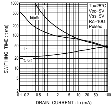
Fig.20 Switching characteristics
