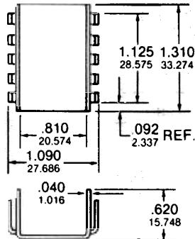
TO-202 CASE 7-292
