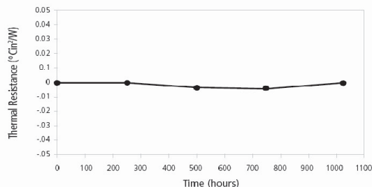
Tgrease 2500 Reliability Thermal Bake @ 125°C
