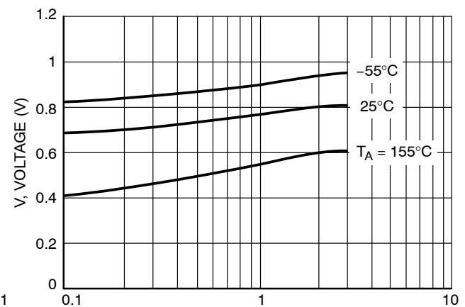
Figure 6. V_{BE(on)} Voltage
