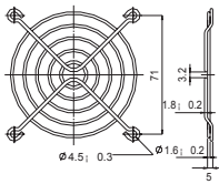
FG-08 For 80mm Fan
