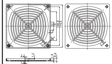
D-1 Finger Guard
