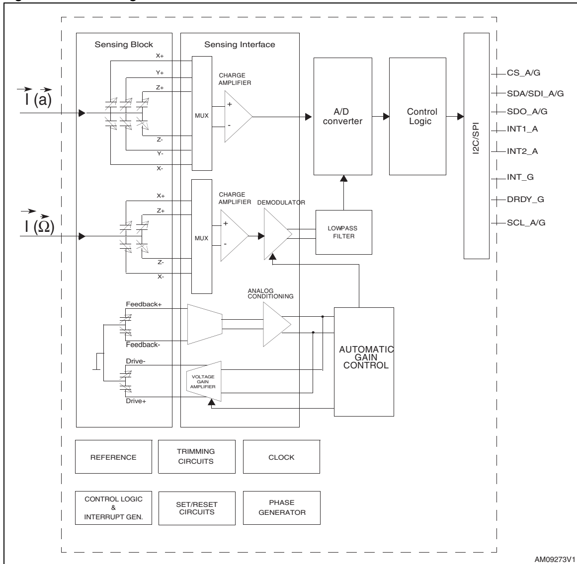
Figure 1. Block diagram
