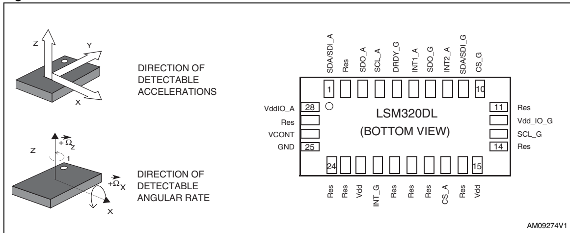
Figure 2. Pin connection
