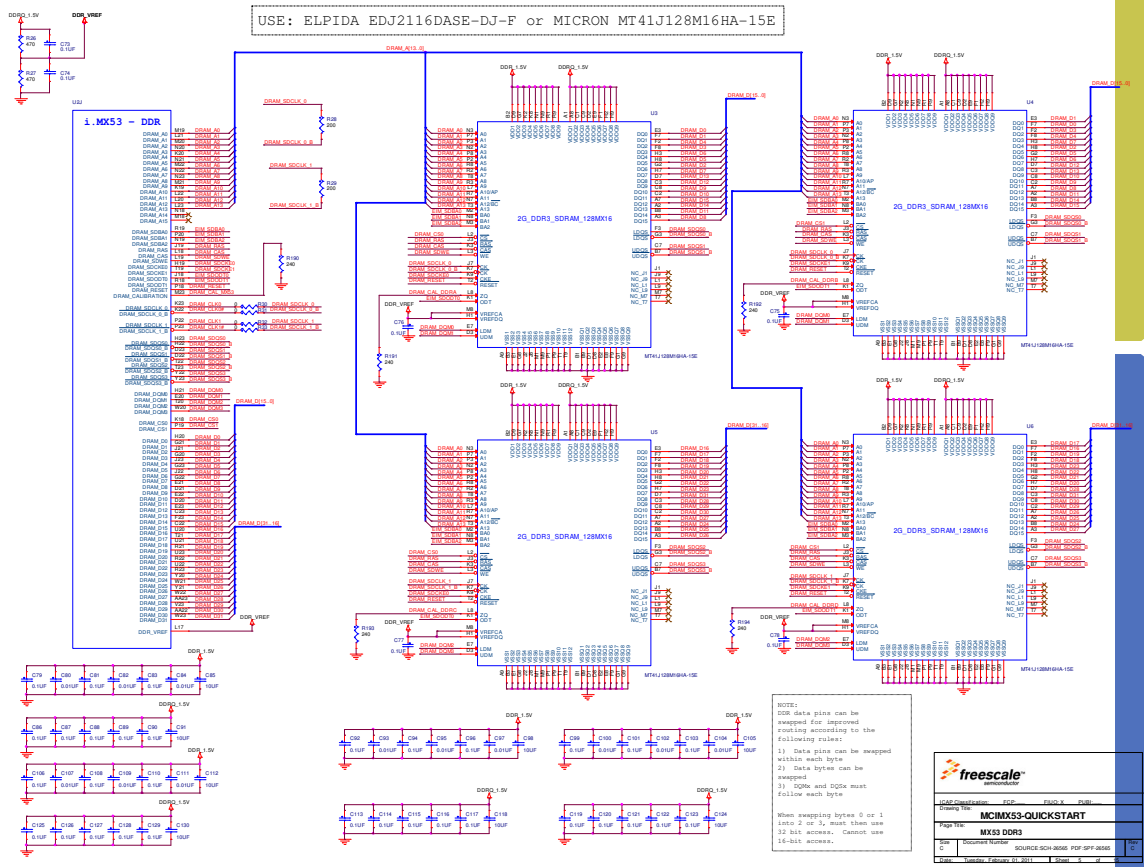
Figure 46. MX53 DDR3 MEMORY
