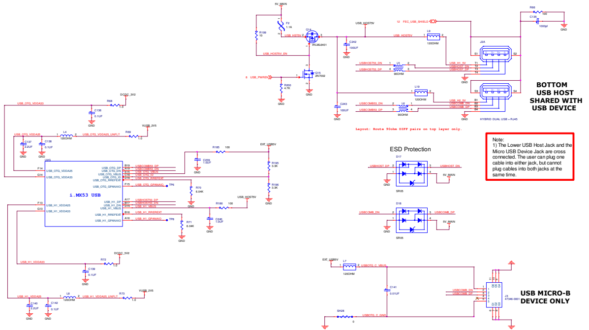
Figure 48. MX53 USB
