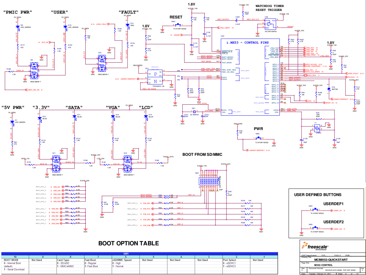
Figure 47. MX53 CONTROL
