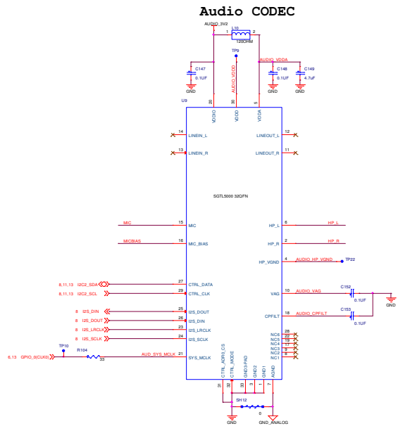
Figure 50. MX53 AUDIO
