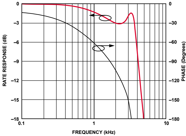
Figure 4. Typical Rate and Phase Response vs. Frequency ( C_{OUT} = 470 pF with a Series RC Low-Pass Filter of 3.3 k \Omega and 22 nF)
