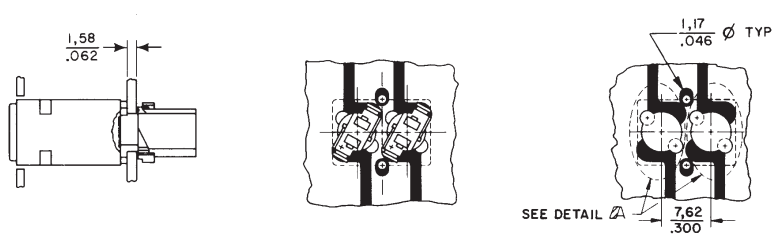
PWB Receptacle Installed (LED or Incandescent Lamp)
