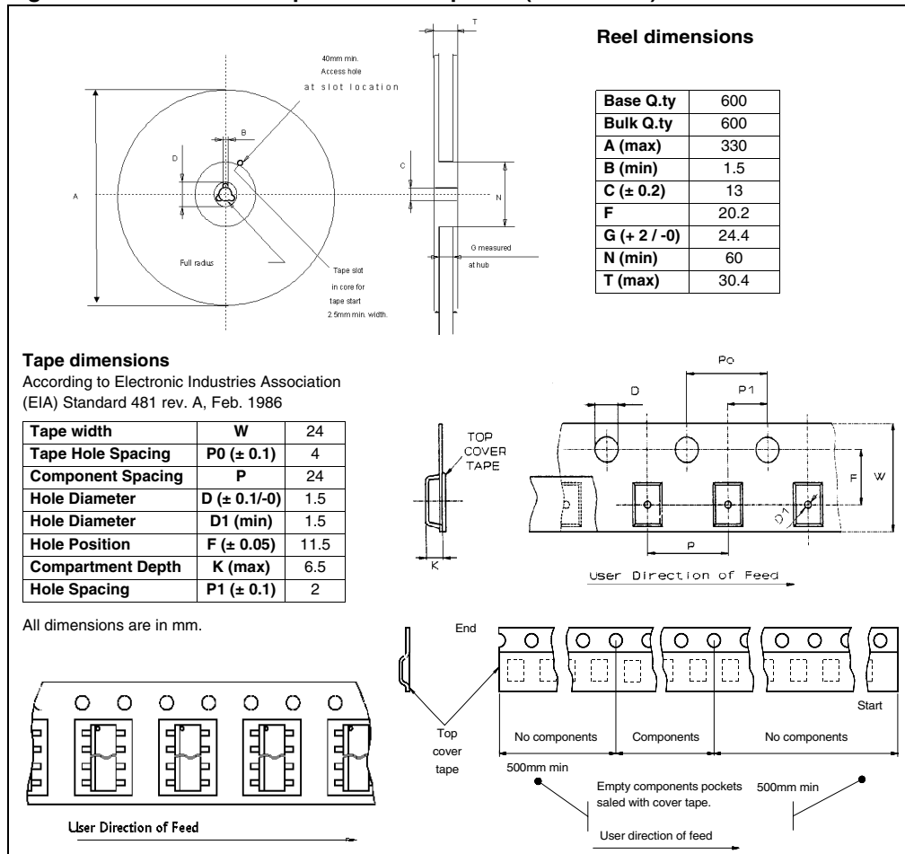
Figure 28. PowerSO-10 tape and reel shipment (suffix “TR”)
