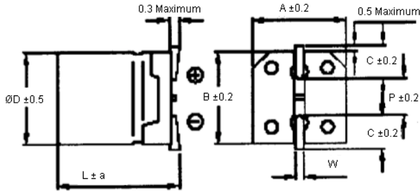
Diagram of Dimensions
