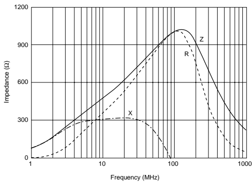
BLM18RK102SN1
