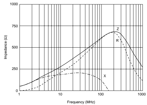
BLM18RK601SN1
