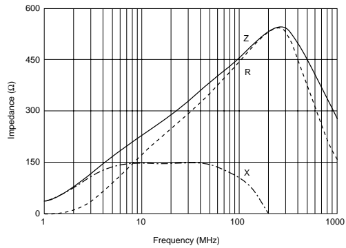
BLM18RK471SN1
