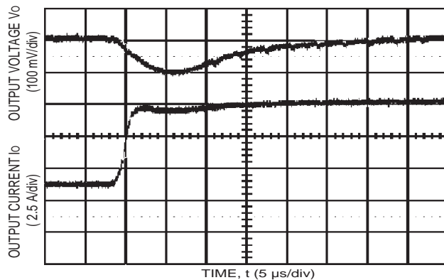
Figure 14. Typical Transient Response to Step Load Change at 2.5 A/ \mu\text{s} from 50% to 100% of I_{O,max} at 3.3 V Input (COUT = 1 \mu\text{F} ceramic, 10 \mu\text{F} Tantalum).
