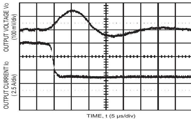
Figure 13. Typical Transient Response to Step Load Change at 2.5 A/ \mu\text{s} from 100% to 50% of I_{O,max} at 3.3 V Input (COUT = 1 \mu\text{F} ceramic, 10 \mu\text{F} Tantalum).
