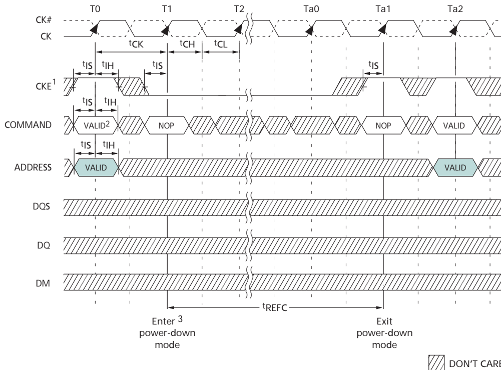
Figure 53: Power-Down Mode
