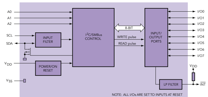
Block diagram
