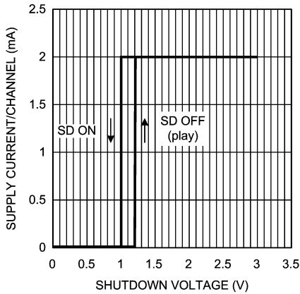
Shutdown Hysteresis Voltage 2.6V
