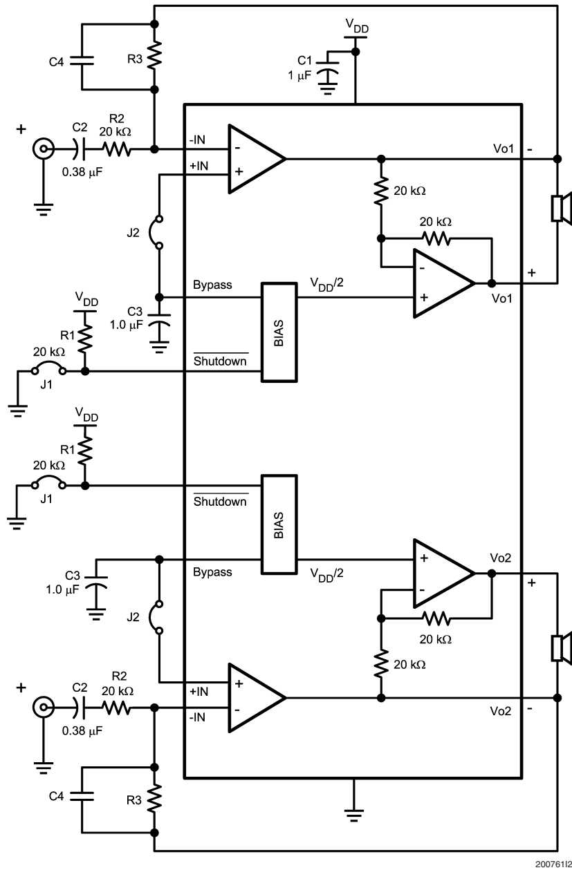
FIGURE 2. Higher Gain Schematic Drawing
