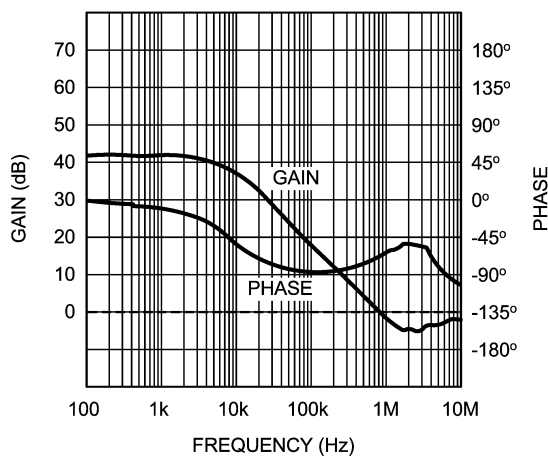
Open Loop Frequency Response, 2.6V
