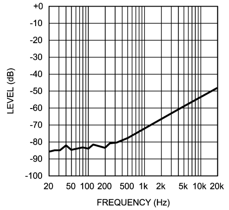
Input Floating
