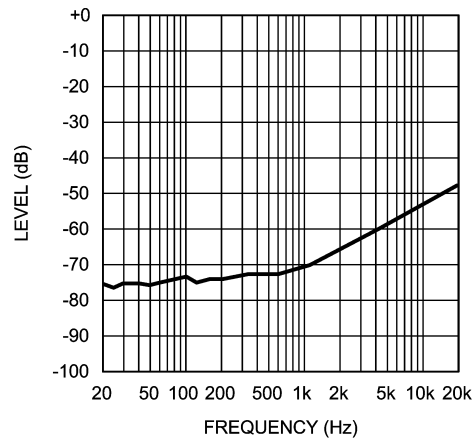
Input Floating
