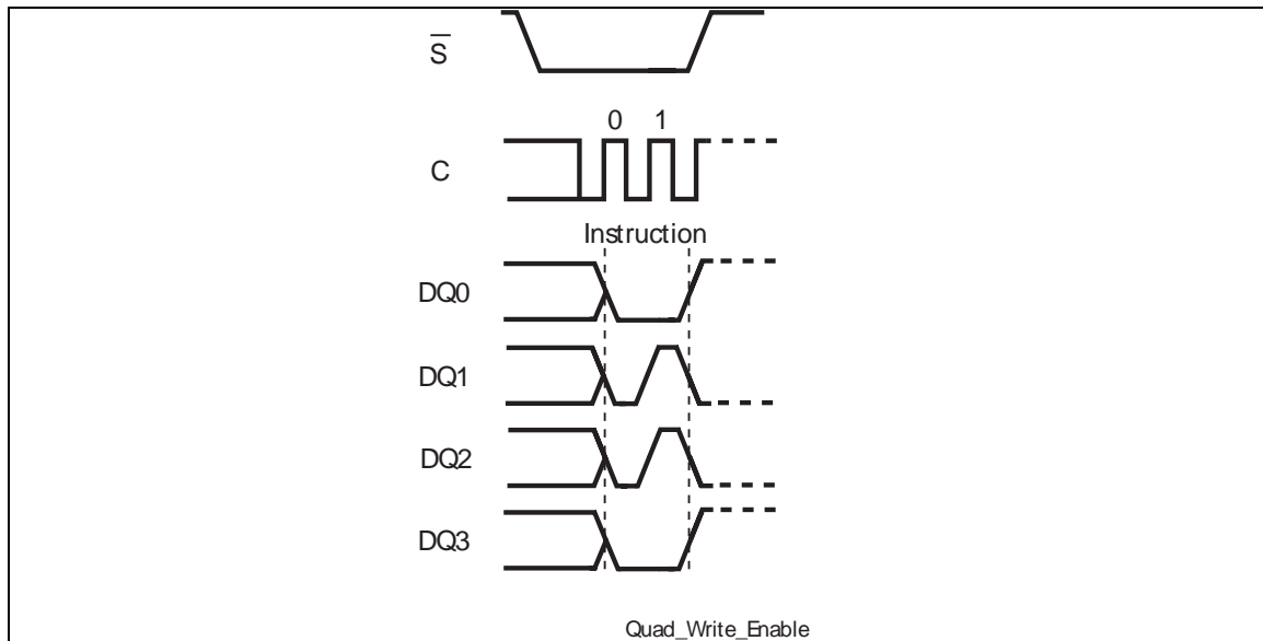
Figure 76. Write Enable instruction sequence QIO-SPI
