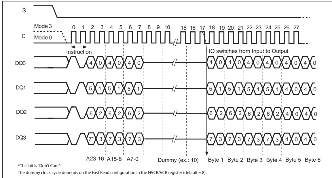
Figure 71. Quad Read Serial Flash Discovery Parameter
