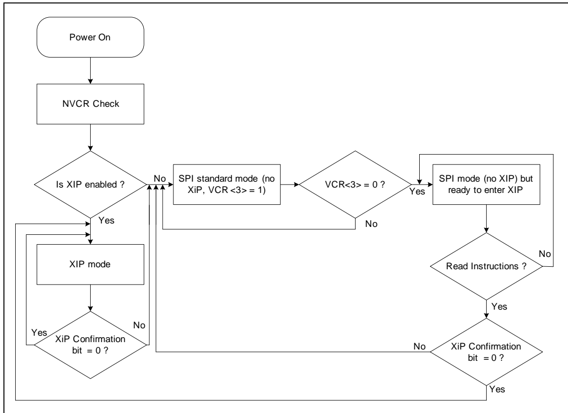
Figure 99. N25Q064 Read functionality Flow Chart
