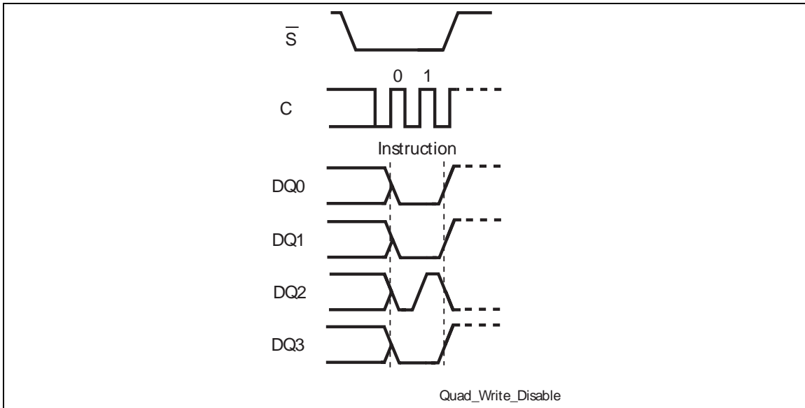
Figure 77. Write Disable instruction sequence QIO-SPI
