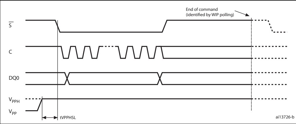
Figure 109. V_{PPH} timing
