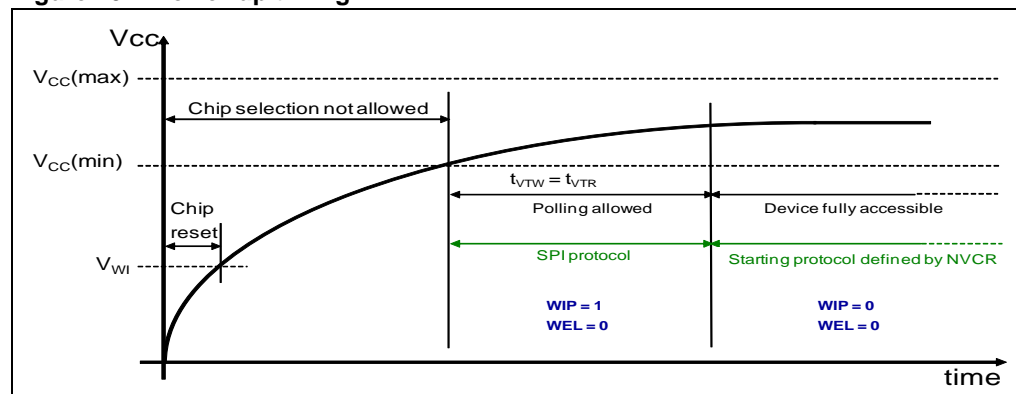
Figure 102. Power-up timing
