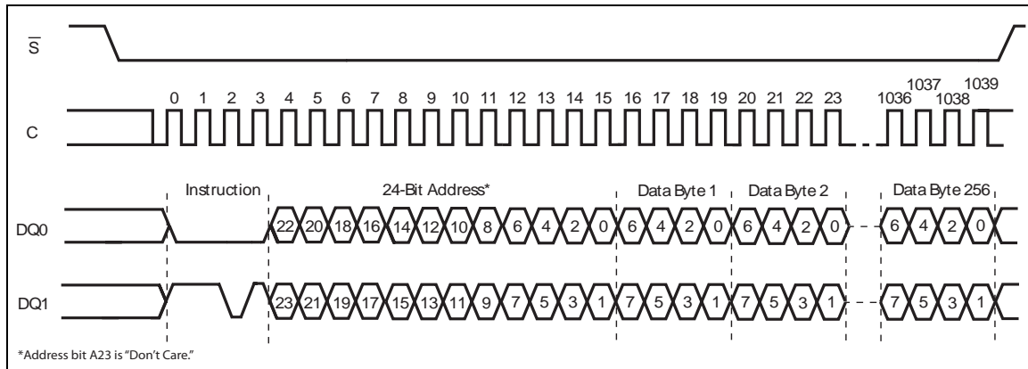
Figure 50. Dual Command Page Program instruction sequence DSP, A2h
