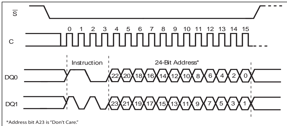
Figure 54. Sector Erase instruction sequence DIO-SPI
