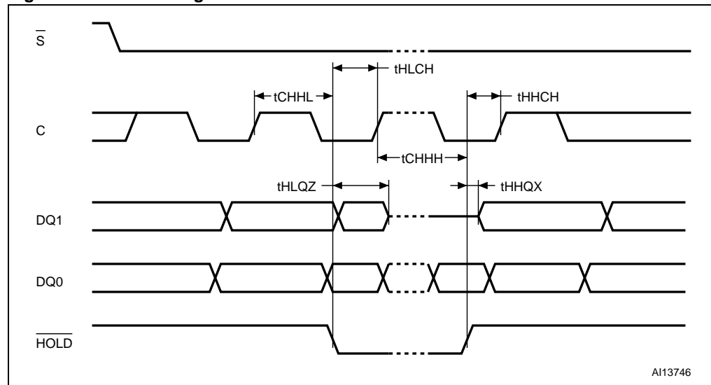
Figure 107. Hold timing
