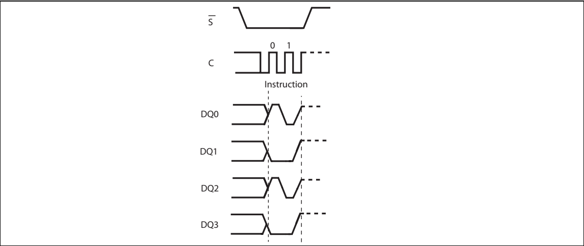
Figure 92. Clear Flag Status Register instruction sequence QIO-SPI
