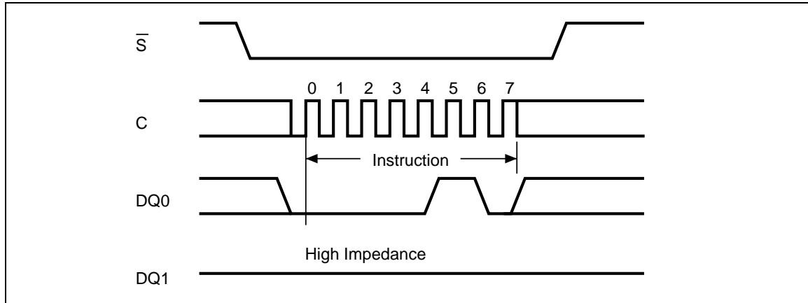
Figure 19. Write Enable instruction sequence
