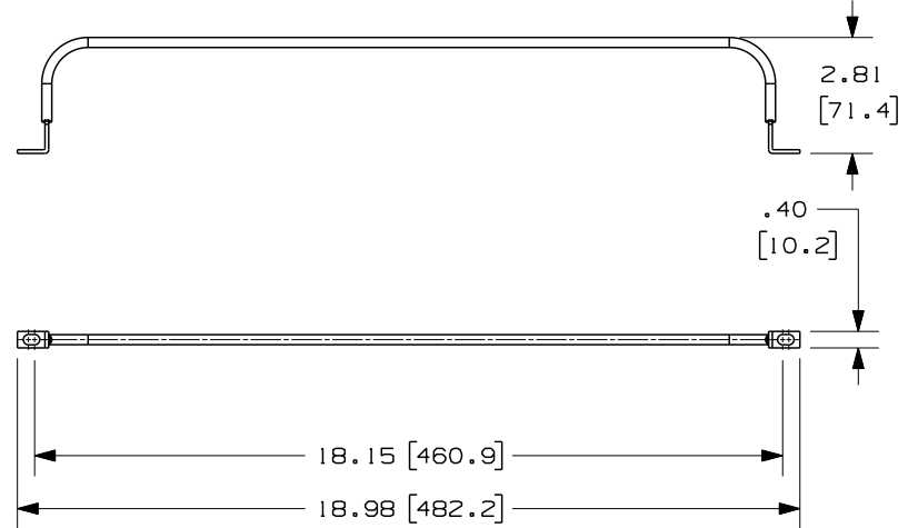
FIGURE 3 STRAIN RELIEF BAR
