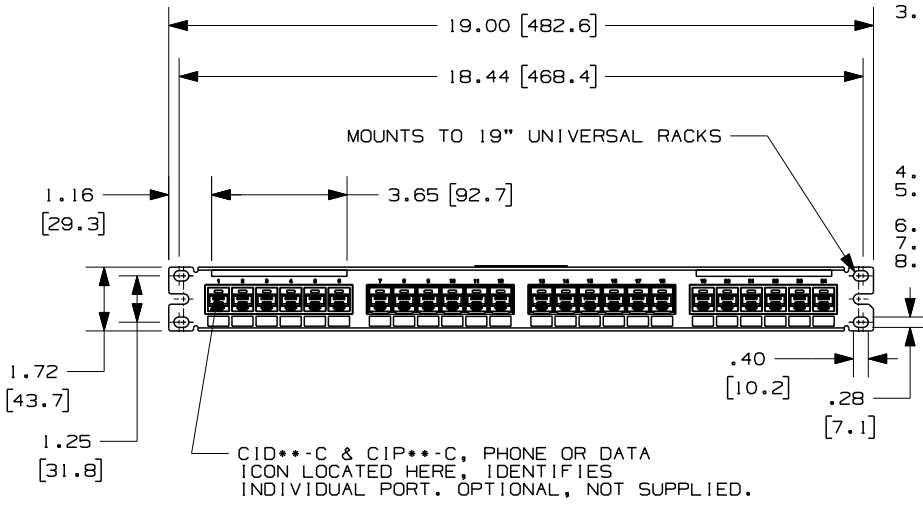
FIGURE 1 DP6 PLUS 24 PORT PATCH PANEL
