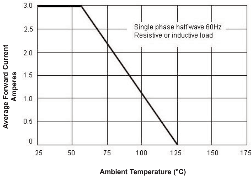
Figure 1 - Forward Current Derating Curve
