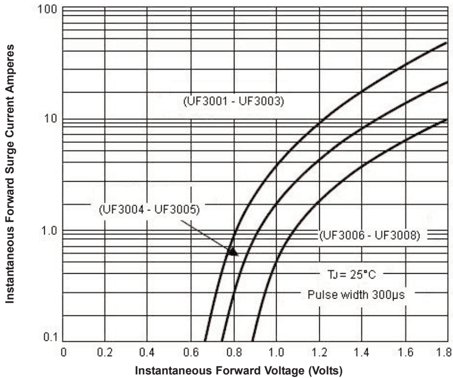
Figure 4 - Typical Forward Characteristics
