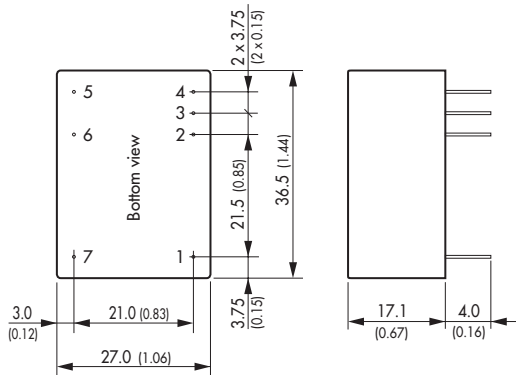
Pin diameter: 0.5 (0.02)
