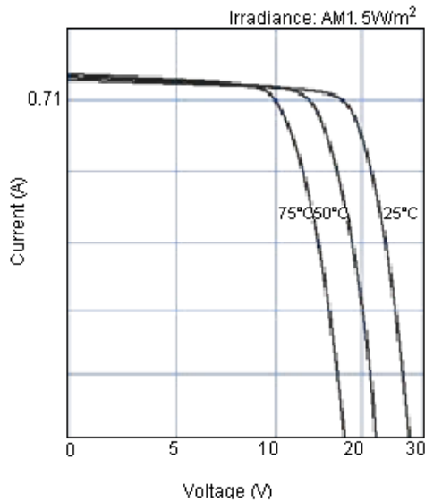
Current-voltage characteristics of photovoltaic Module SP12 at various cell temperatures
