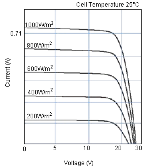
Current-voltage characteristics of photovoltaic Module SP12 at various irradiance levels
