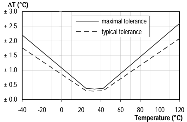
Figure 3 Maximal tolerance for temperature sensor in °C.
