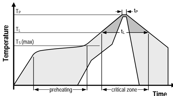
Figure 9 Soldering profile according to JEDEC standard. T_P <= 260^\circ\text{C} and t_P < 40\text{sec} for Pb-free assembly. T_L < 220^\circ\text{C} and t_L < 150\text{sec} . Ramp-up/down speeds shall be < 5^\circ\text{C}/\text{sec} .
