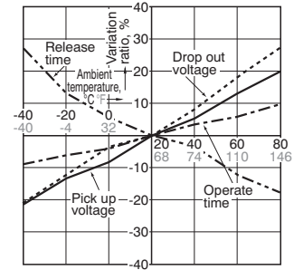
1.-(3) Ambient temperature characteristics (80A type)
