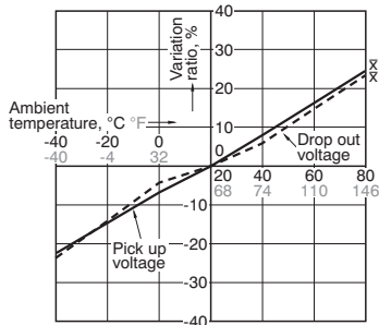
1.-(1) Ambient temperature characteristics (10A type)
