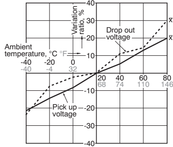
1.-(2) Ambient temperature characteristics (60A type)
