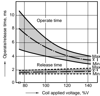
2. Operate/release time Sample: 25 pcs., JS1-12V-F
