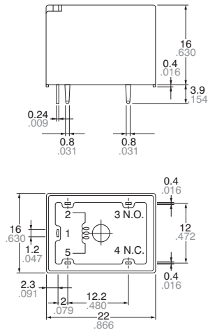
Schematic (Bottom view)
