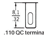
.110 QC terminal
