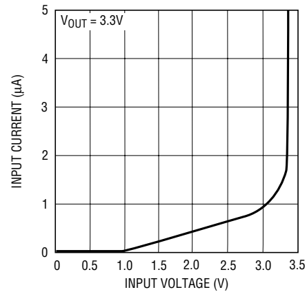
Figure 4. Input Current
