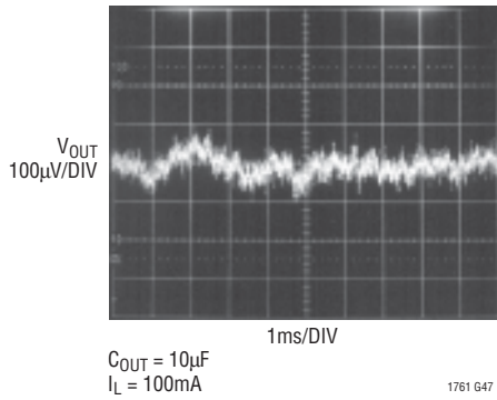
LT1761-5 10Hz to 100kHz Output Noise C_{\text{BYP}} = 1000\text{pF}
