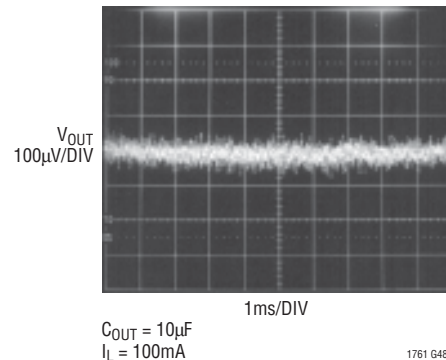
LT1761-5 10Hz to 100kHz Output Noise C_{\text{BYP}} = 0.01\mu\text{F}
