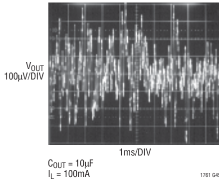
LT1761-5 10Hz to 100kHz Output Noise C_{\text{BYP}} = 0
