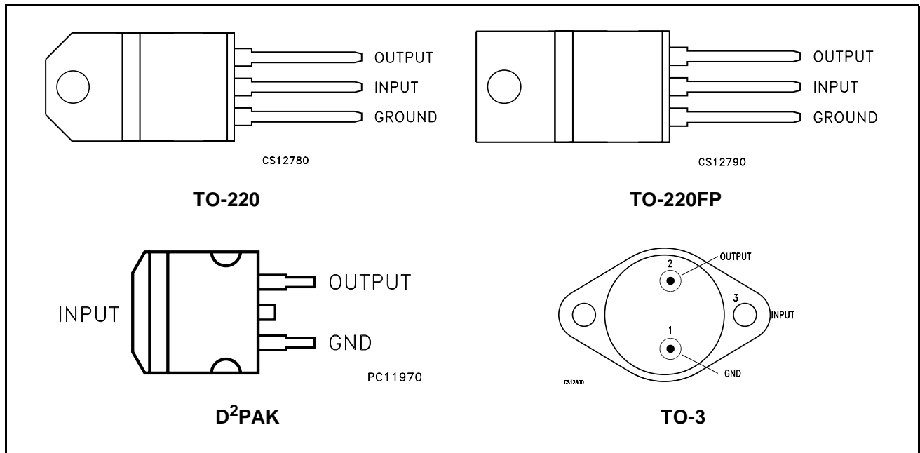
Figure 2: Connection Diagram (top view)
