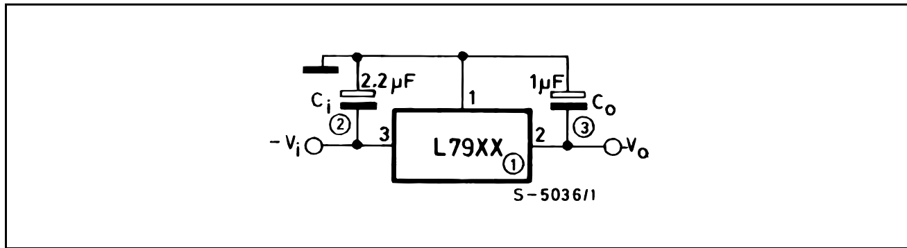
Figure 4: Fixed Output Regulator
