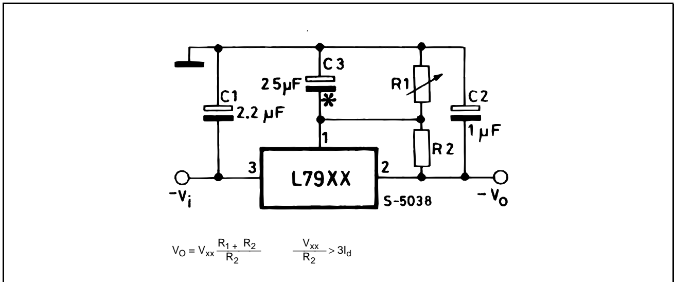
Figure 6: Circuit for Increasing Output Voltage
