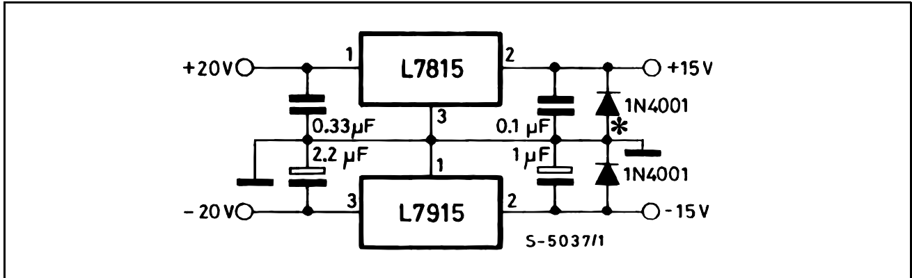
Figure 5: Split Power Supply ( \pm 15V/1A )
