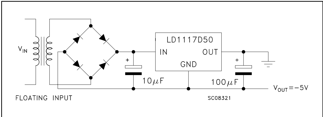
Figure 5: Active Terminator for SCSI-2 BUS
