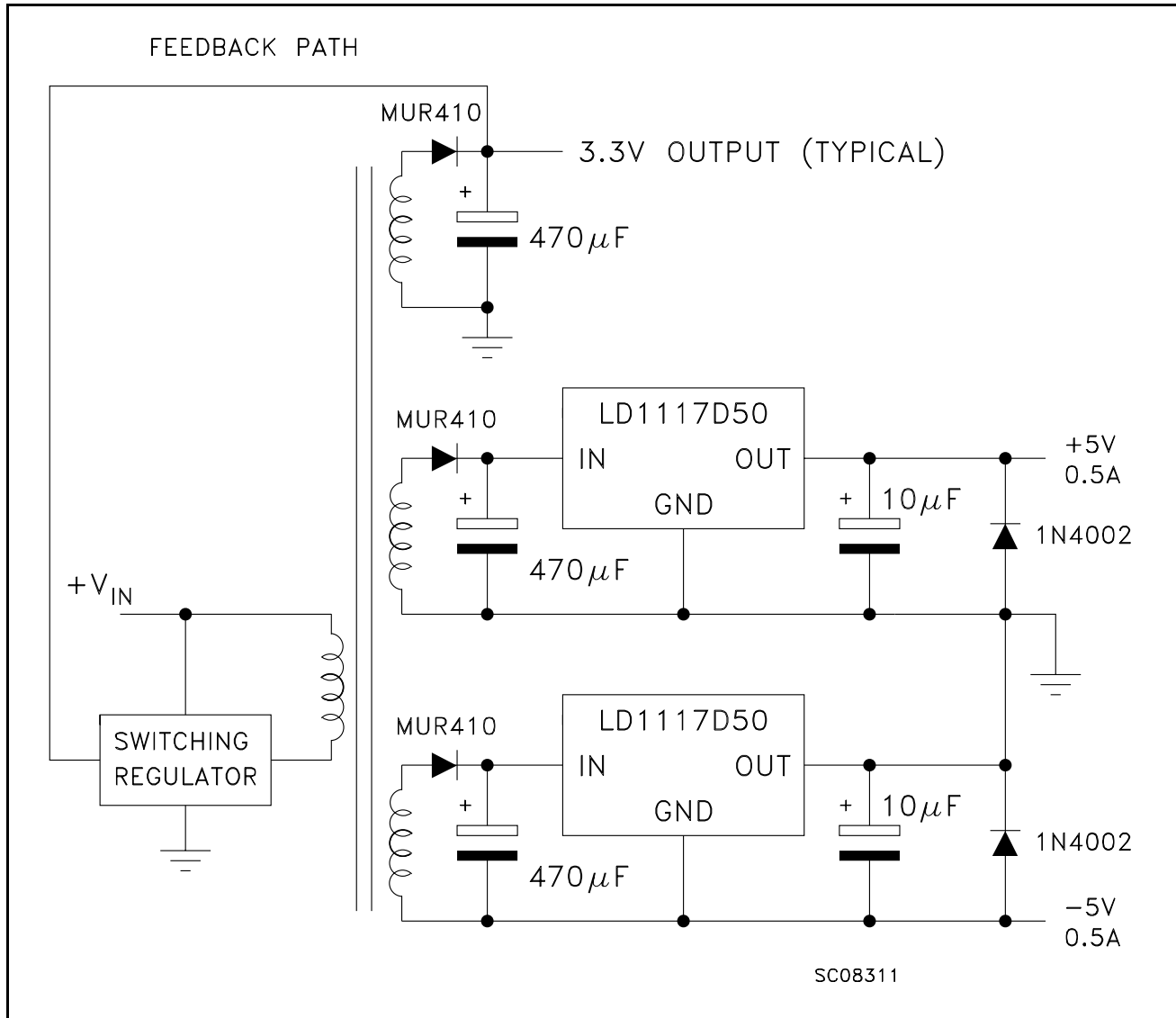
Figure 9: Post-Regulated Dual Supply
