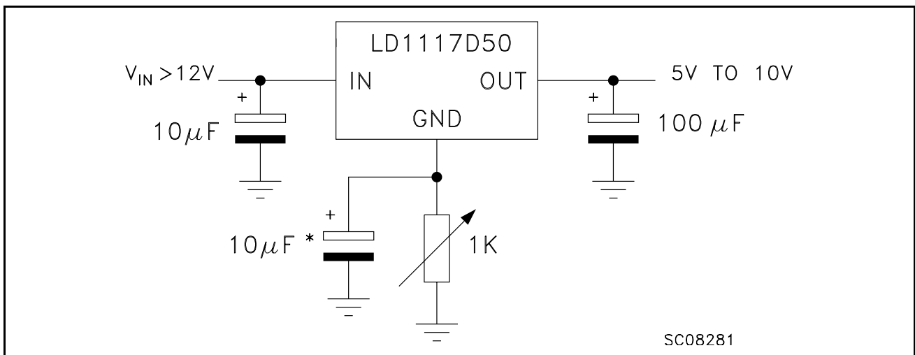
Figure 6: Circuit for Increasing Output Voltage
