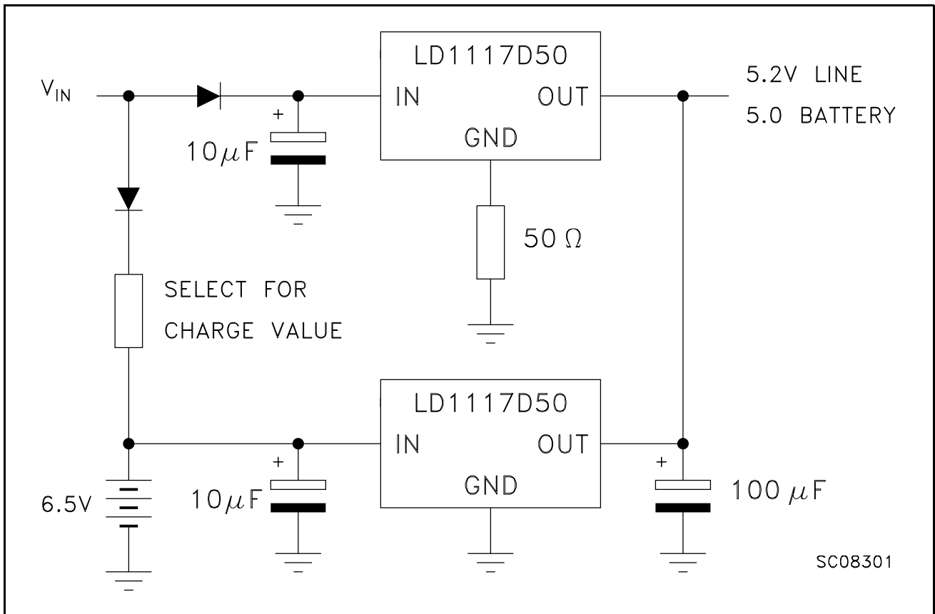
Figure 8: Battery Backed-up Regulated Supply
