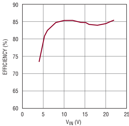
Efficiency vs V_{IN} , Buck-Boost Mode, 12.6V at 350mA LED String
