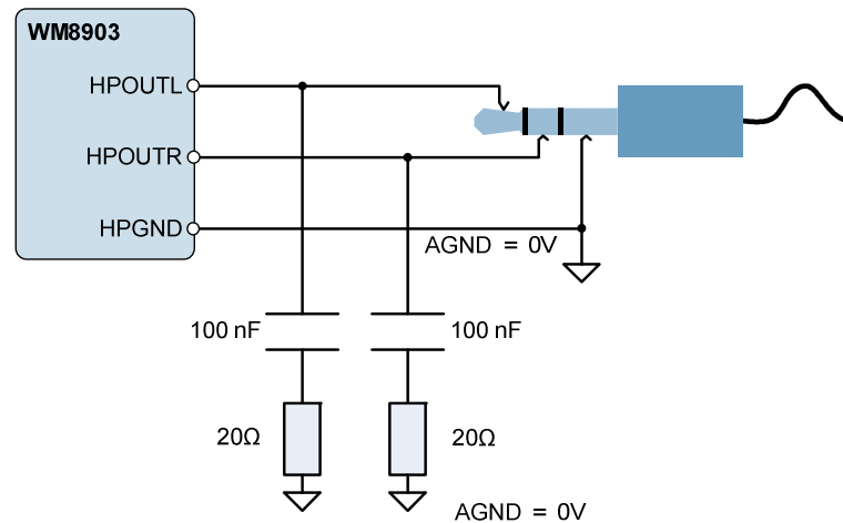
Figure 34 Zobel Network Components for HPOUTL, HPOUTR, LINEOUTL and LINEOUTR
