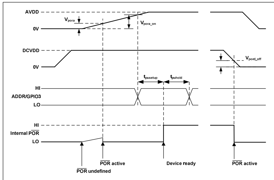
Figure 66 Power On Reset timing - DCVDD enabled first
