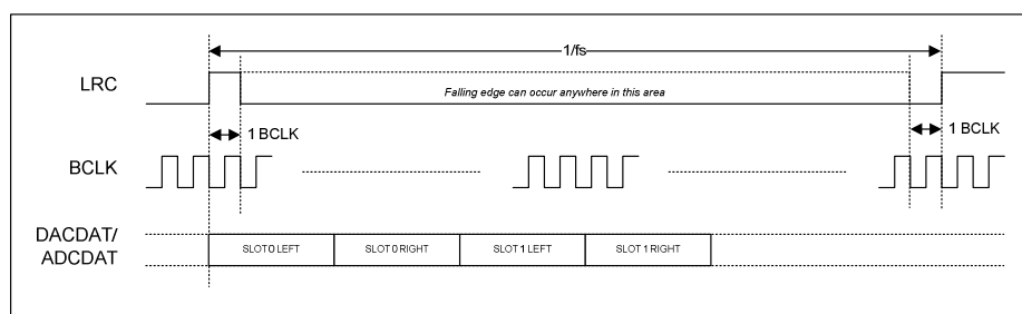
Figure 52 TDM in DSP Mode B
