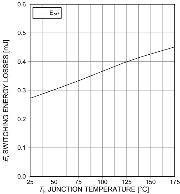
Figure 15. Typical switching energy losses as a function of junction temperature (inductive load, V_{CE}=400\text{V} , V_{GE}=15/0\text{V} , I_c=10\text{A} , R_G=23\Omega , Dynamic test circuit in Figure E)
