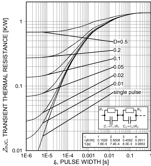
Figure 21. Diode transient thermal resistance ( D = t_p/T )
