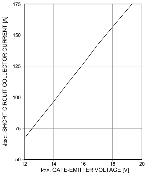
Figure 19. Typical short circuit collector current as a function of gate-emitter voltage ( V_{CE}\leq 400V , start at T_{vj}=25^\circ C )
