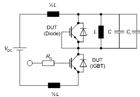
Figure E. Dynamic test circuit Leakage inductance L = 180\text{nH} , Stray capacitor C_o = 40\text{pF} , Relief capacitor C_r = 1\text{nF} (only for ZVT switching)
