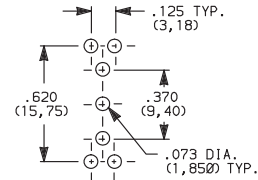
8161SH9_BE2 SPDT
