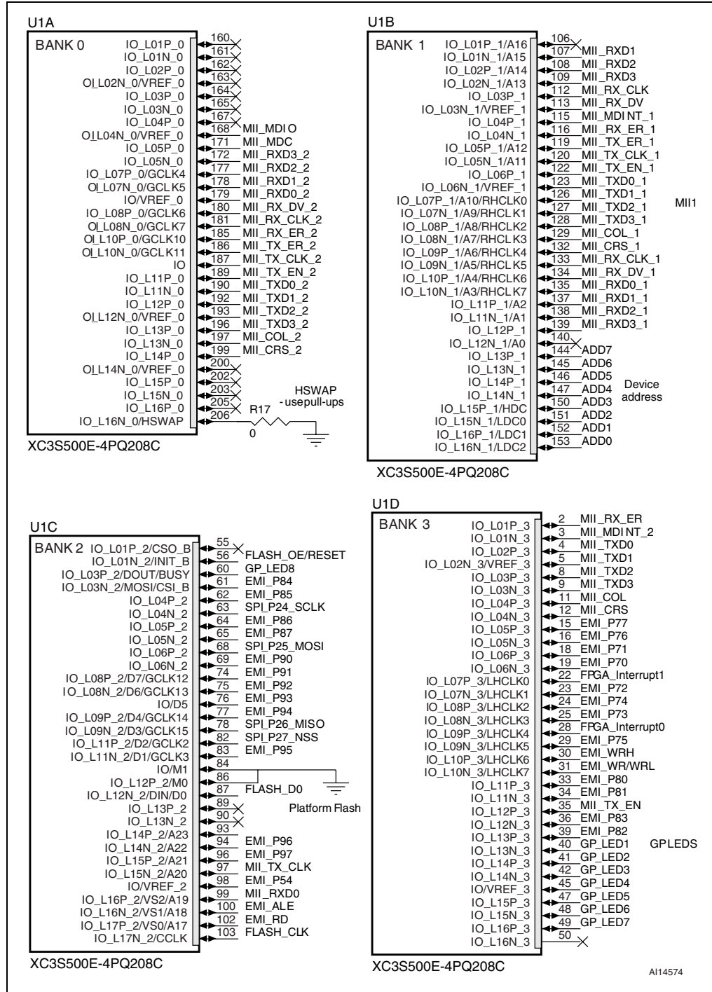
Figure 4. FPGA schematic
