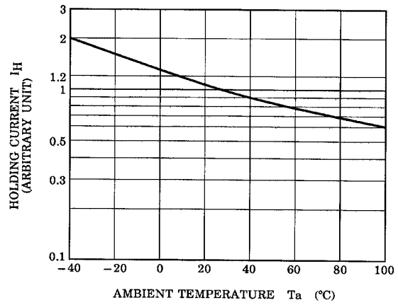
NORMALIZED I_H - T_a
