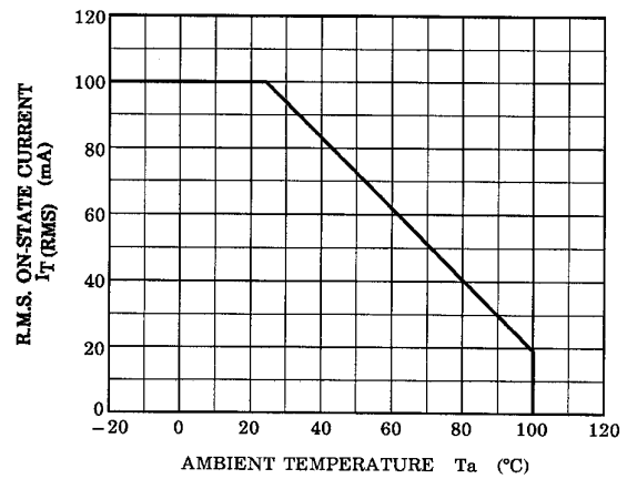
I_T (RMS) - T_a
