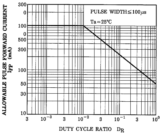
I_{FP} - D_R
