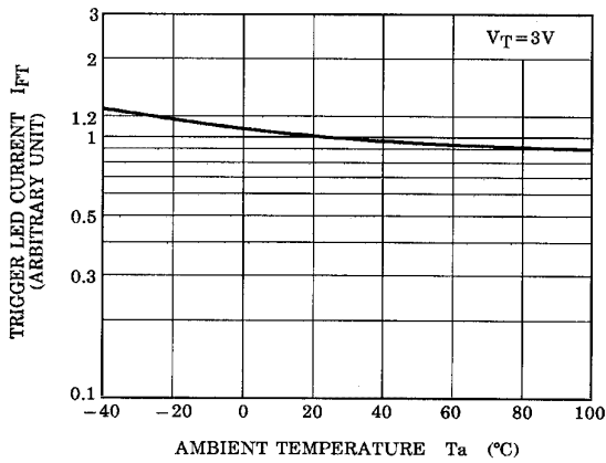
NORMALIZED I_{FT} - T_a
