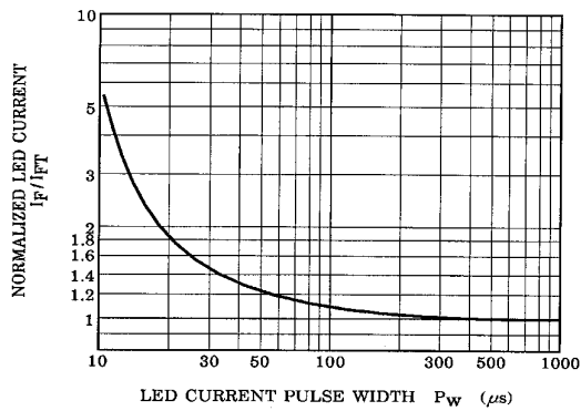
NORMALIZED LED CURRENT - LED CURRENT PULSE WIDTH
