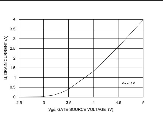
Figure 4. Drain current vs. gate voltage
