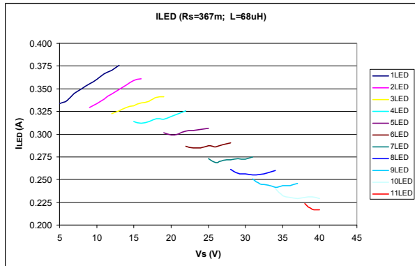
ILD4035_I_LED_367m_68u.vsd
