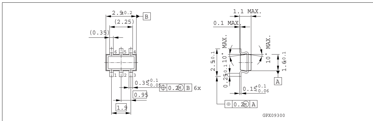
Figure 10 Package Outline
