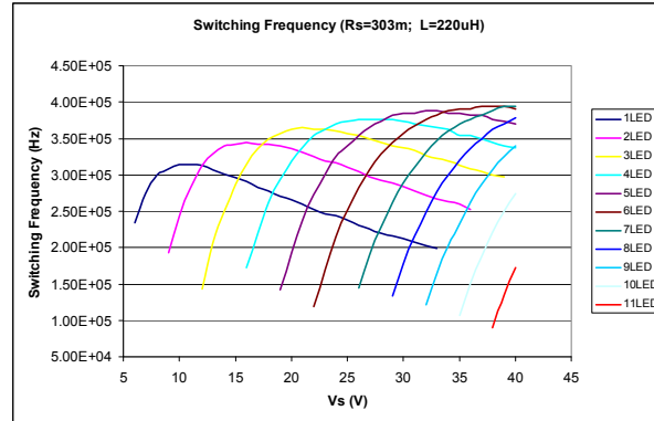
ILD4035_Switching_Frequency_303m_220u.vsd
