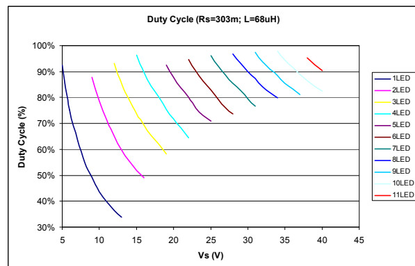
ILD4035_Duty_Cycle_303m_68u.vsd
