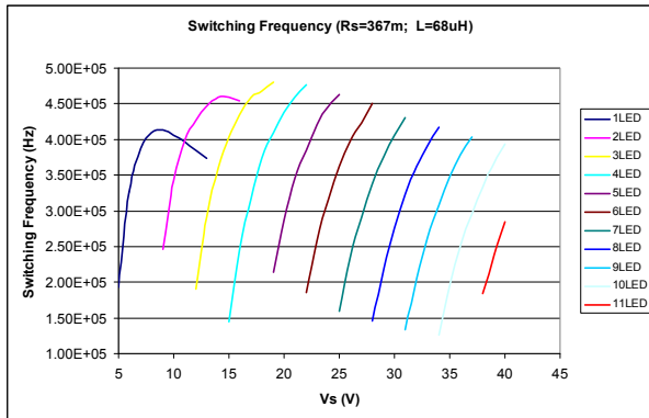
ILD4035_Switching_Frequency_367m_68u.vsd
