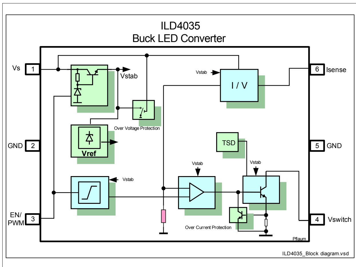
Figure 1 Block Diagram
