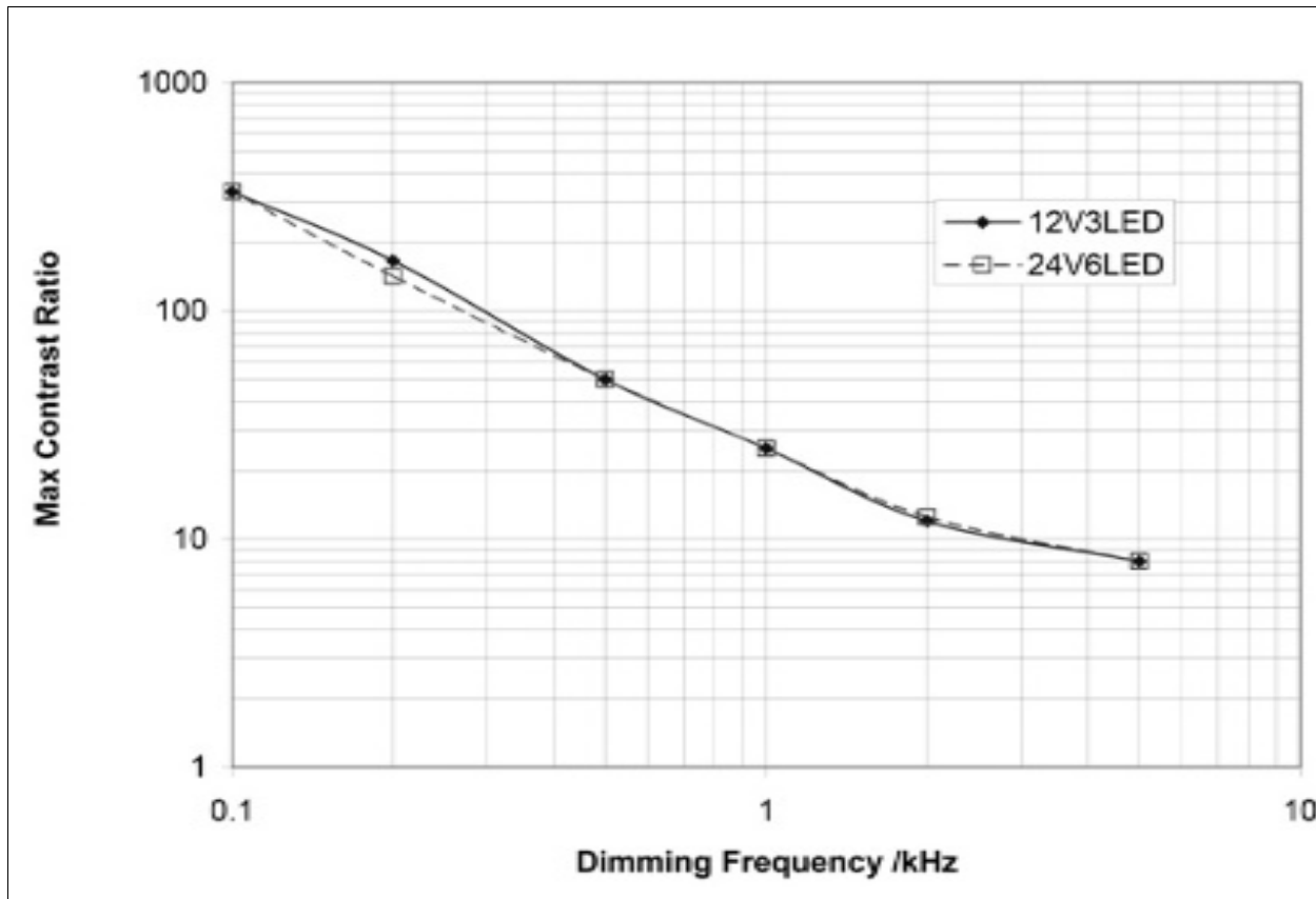
Figure 7 ILD4035; PWM Dimming
