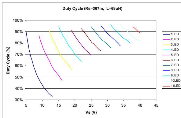
ILD4035_Duty_Cycle_367m_68u.vsd
