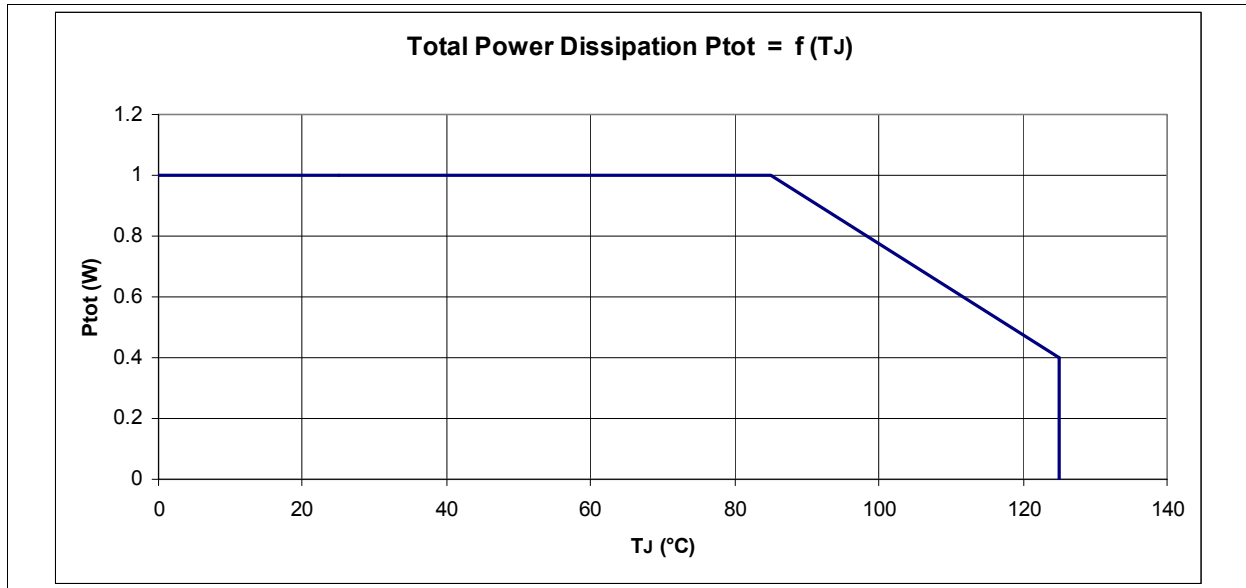
Figure 2 ILD4035; Total Power Dissipation
