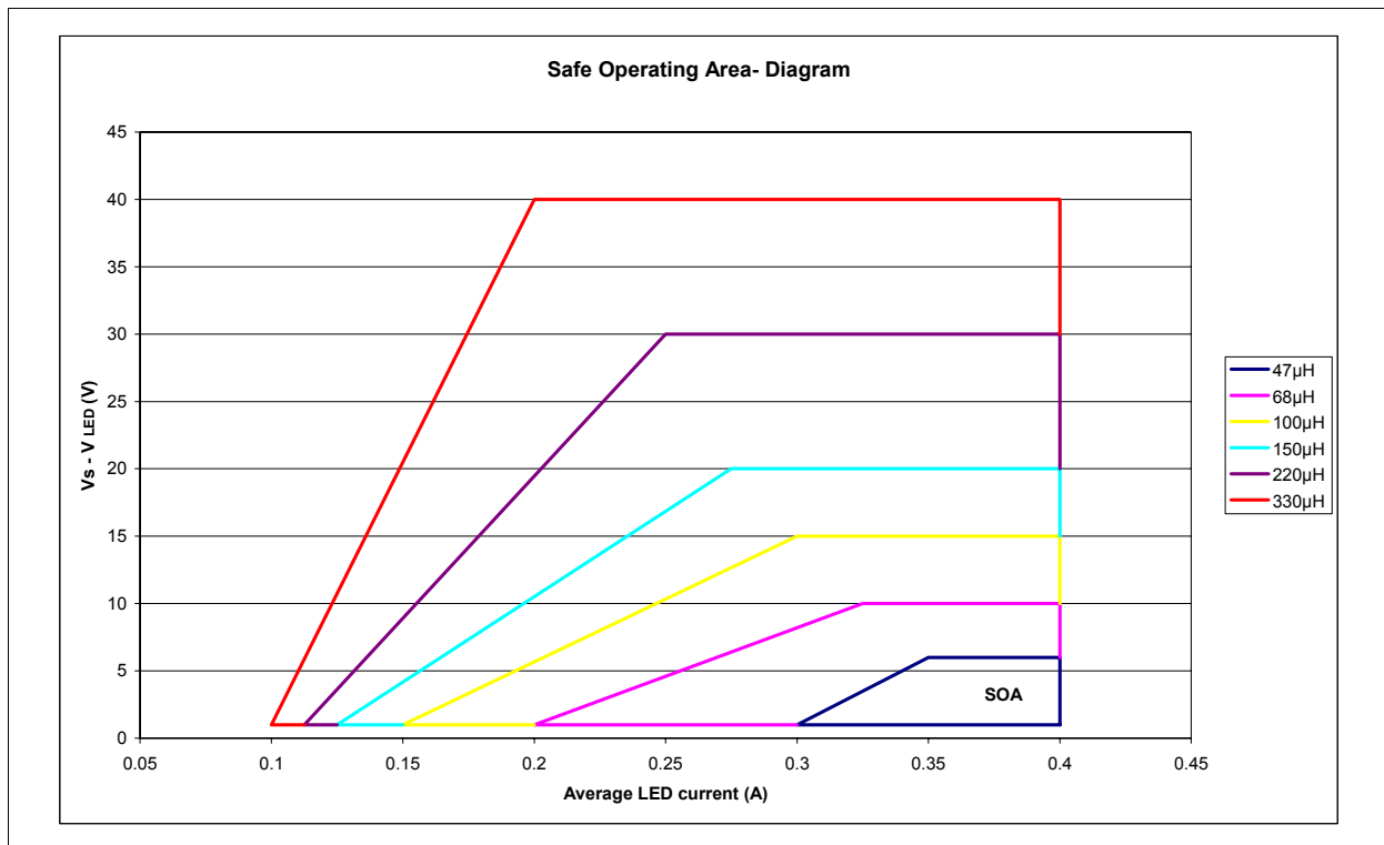
Figure 3 ILD4035; Safe Operating Area
