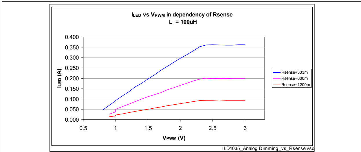
Figure 6 ILD4035; Analog Voltage Dimming with Different Rsense
