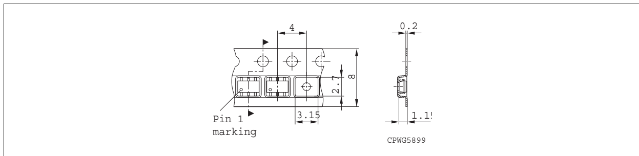
Figure 11 Tape Dimensions
