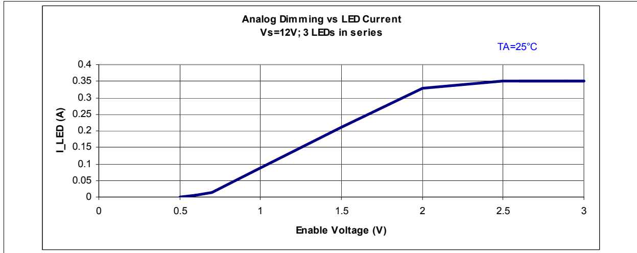
Figure 5 ILD4035; Analog Voltage Dimming
