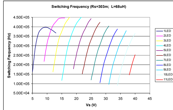
ILD4035_Switching_Frequency_303m_68u.vsd
