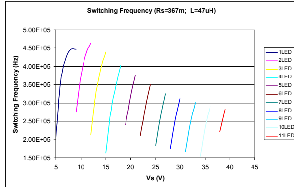
ILD4035_Switching_Frequency_367m_47u.vsd
