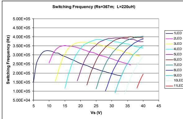
ILD4035_Switching_Frequency_367m_220u.vsd
