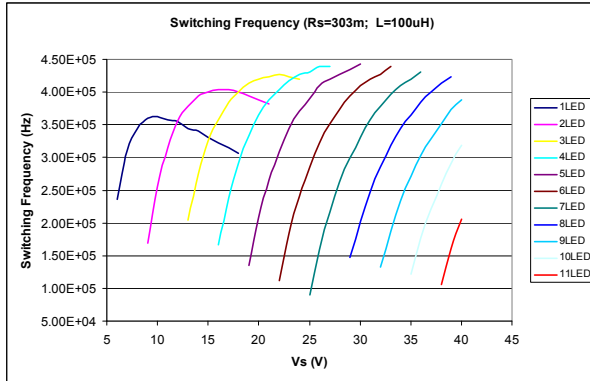
ILD4035_Switching_Frequency_303m_100u.vsd
