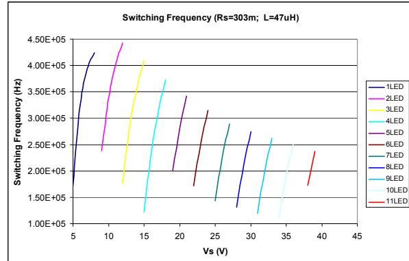
ILD4035_Switching_Frequency_303m_47u.vsd
