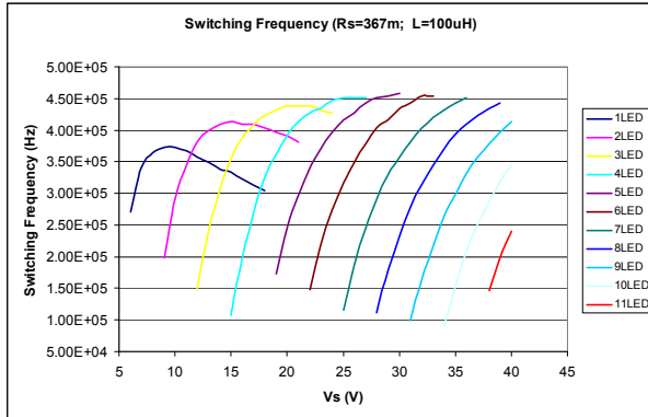
ILD4035_Switching_Frequency_367m_100u.vsd
