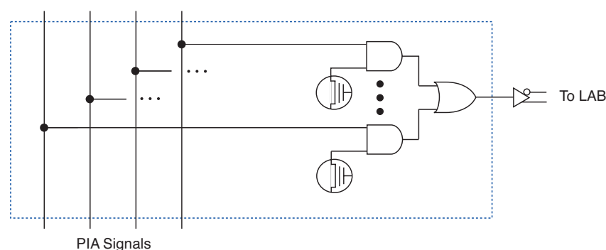
Figure 7. PIA Routing
