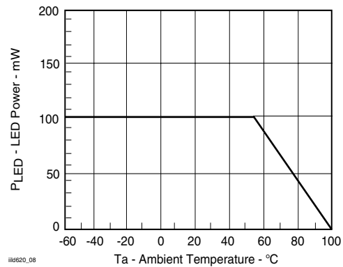
Figure 8. Maximum LED Power Dissipation
