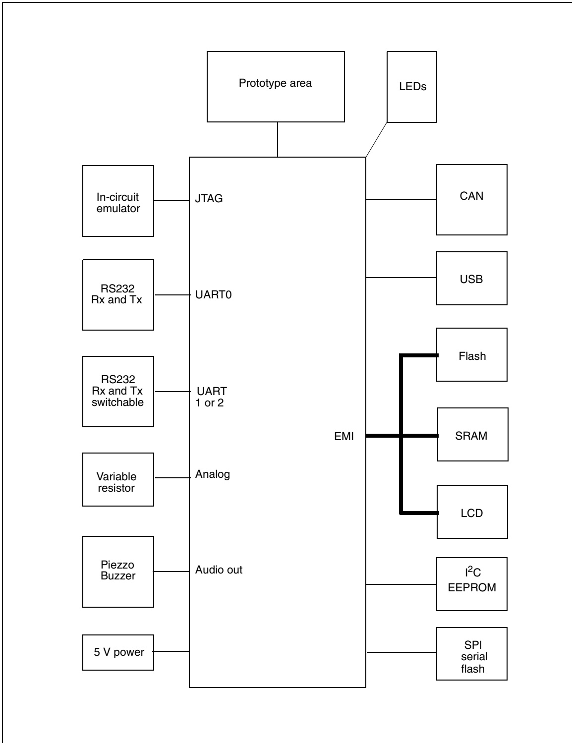
Figure 2. STR710-EVAL board system block diagram
