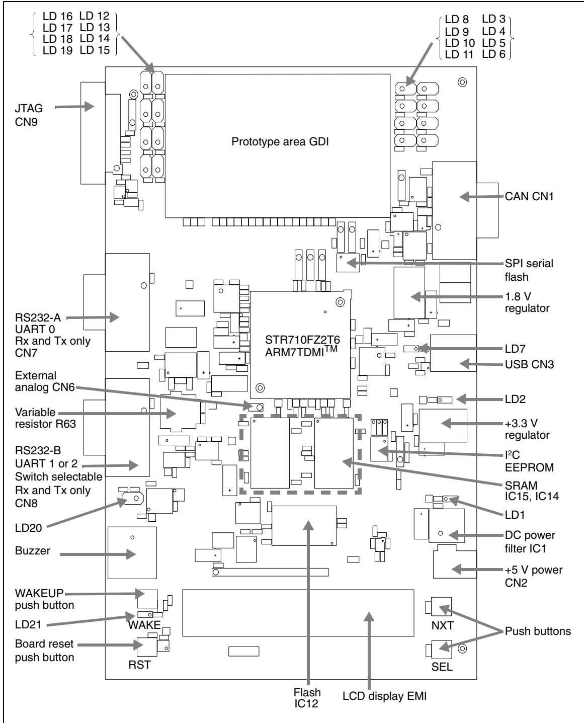
Figure 1. STR710-EVAL board layout block diagram
