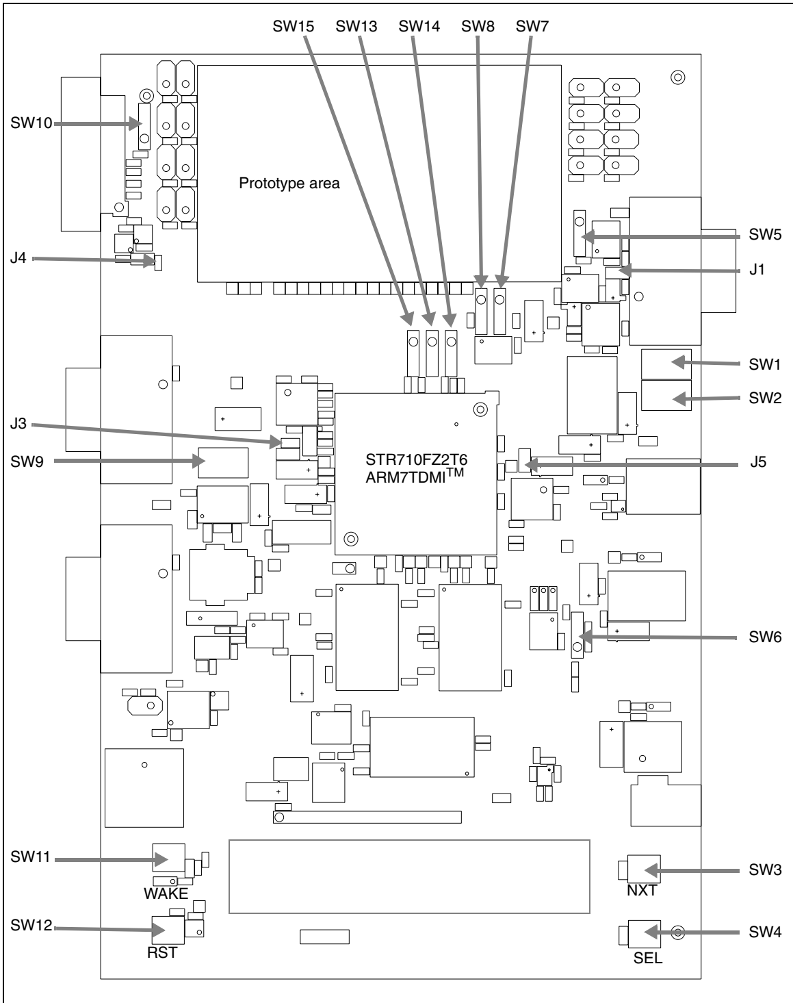
Figure 3. Option jumpers, resistors and switches
