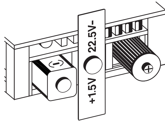
Figure 6-1: Battery Replacement
