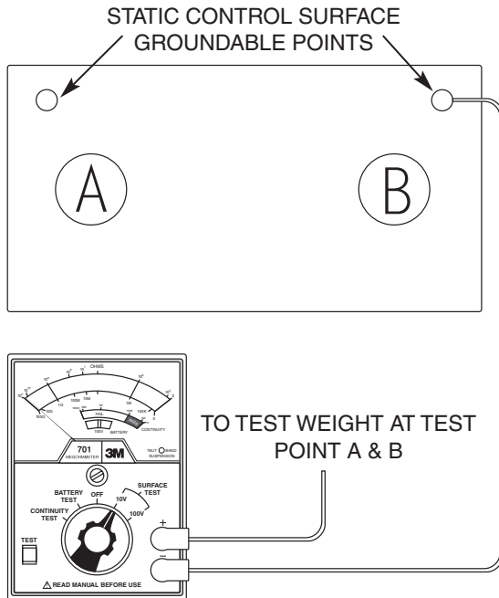
Figure 5-4: Material Evaluation Surface to Groundable Point Test
