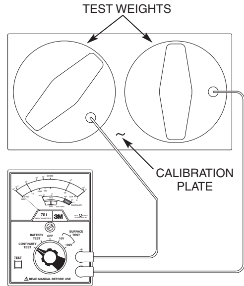
Figure 4-1: Continuity Test
