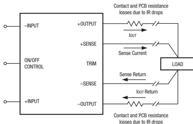
Figure 10. Remote Sense Circuit Configuration
